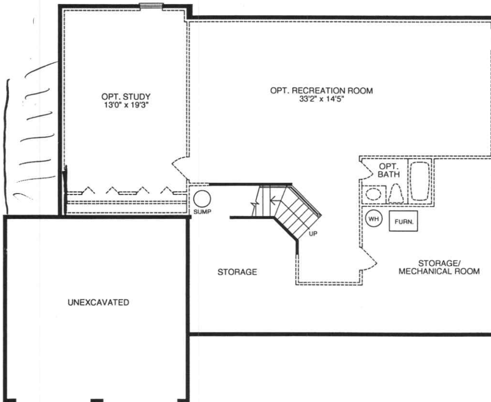
BASEMENT PLAN
