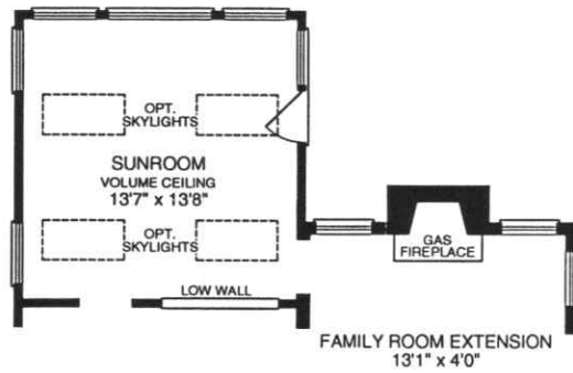
PARTIAL FIRST FLOOR PLAN W/ OPT. SUNROOM & OPT. FAMILY ROOM EXTENSION
