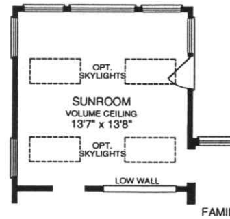
PARTIAL FIRST FLOOR PLAN W/ OPT. SUNROOM & OPT. FAMILY ROOM
